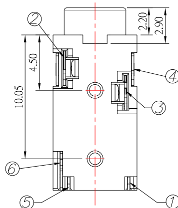
(Ø3.50mm 4 POLE PLUG DETAIL DRAWING)
